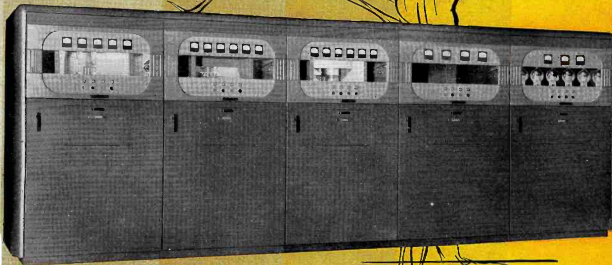
Collins 736A-1 50,000 watt FM transmitter
